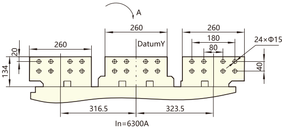
Busbar size and interval
