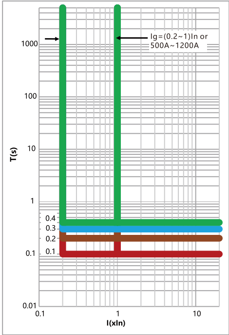
Fig.2 Asymmetrical earth fault protection curves
